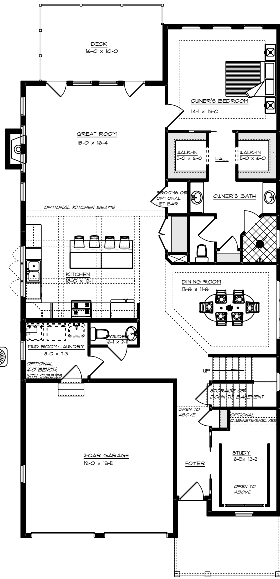
STANDARD FIRST FLOOR PLAN
