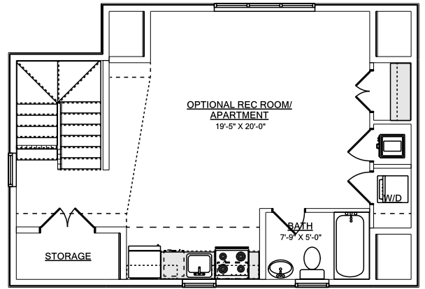
SECOND FLOOR OPTION
