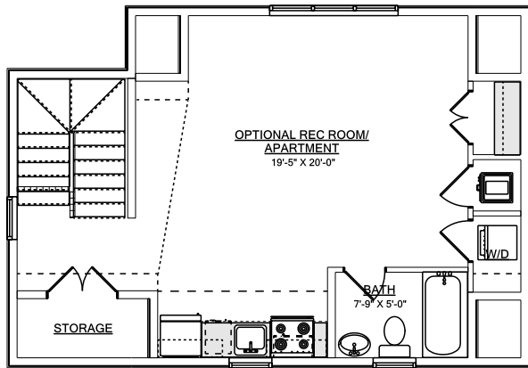
SECOND FLOOR OPTION
