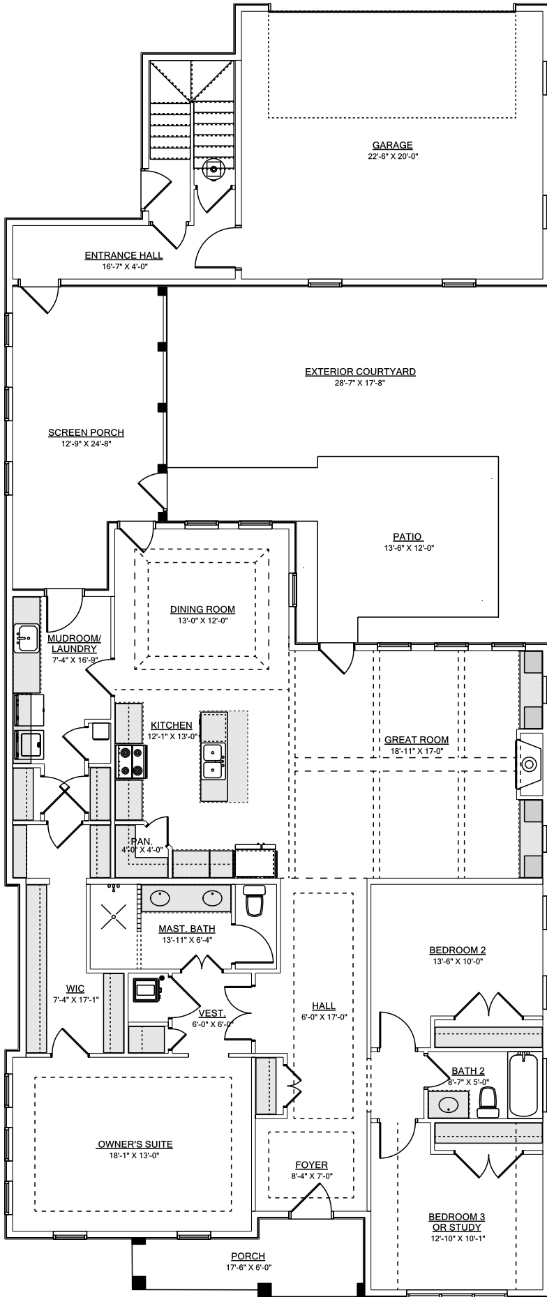
FLOOR PLAN
