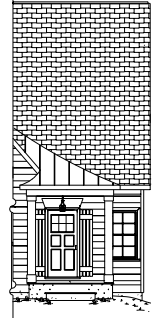
FRONT ELEVATION AND SLIGHT OPTION
