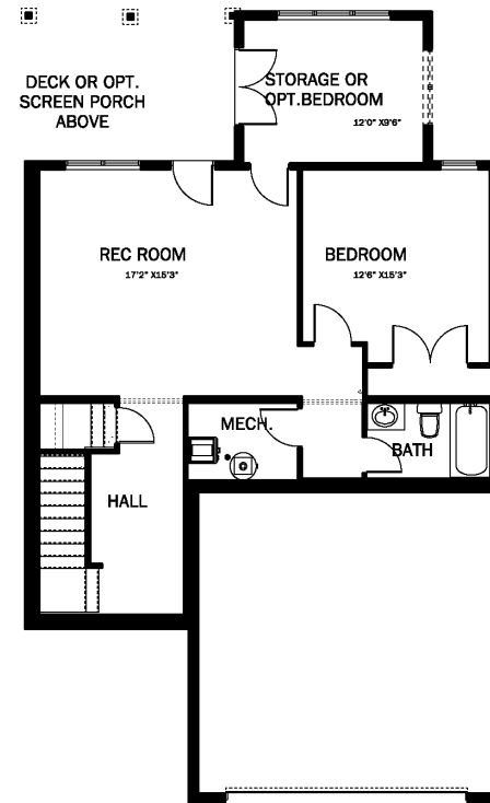
BASEMENT WITH OPT. DINING EXTENSION
