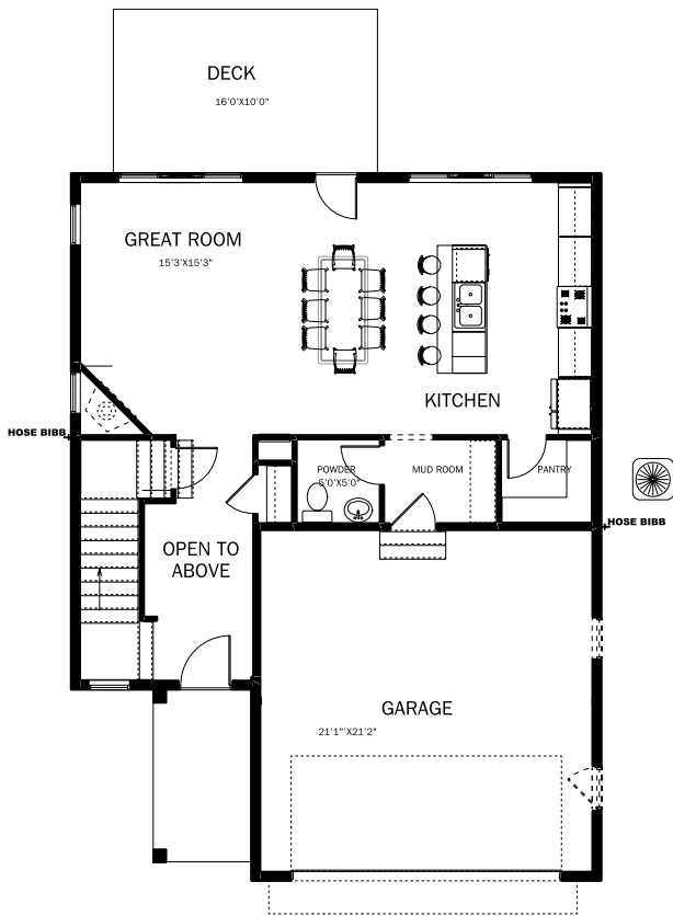
1st. FLOOR ON BASEMENT
